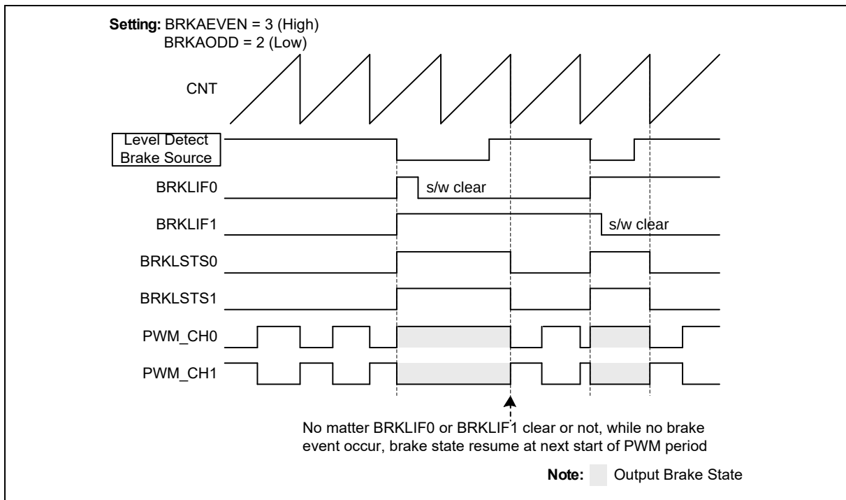
Figure 6.10-27 Level Detector Waveform for PWMx_CH0 and PWMx_CH1 Pair
