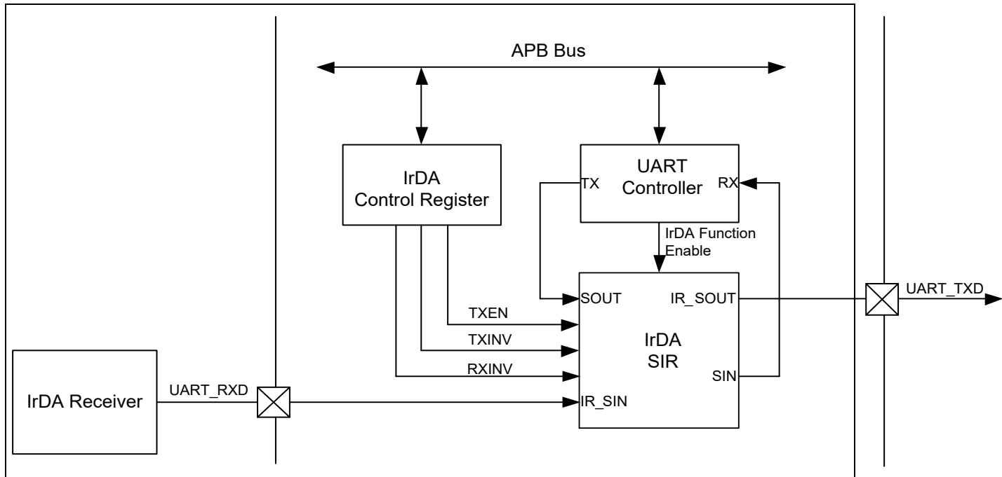
Figure 6.11-15 IrDA Control Block Diagram
