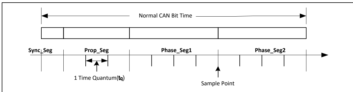
Figure 6.16-7 Bit Timing
